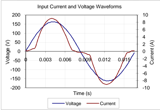
Input AC Current Waveform (ITHD = 33.57%, 50% Load)
